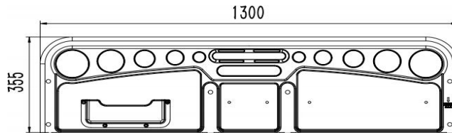
侧护栏: 1300mm × 355mm × 30mm
