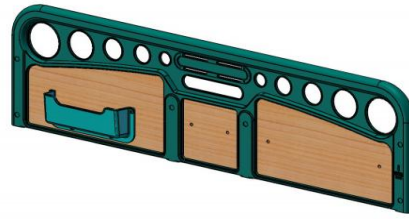
侧护栏: 1300mm × 355mm × 30mm
